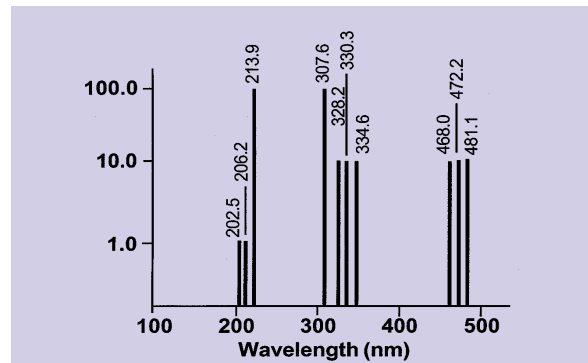
ZINC SPECTRUM
