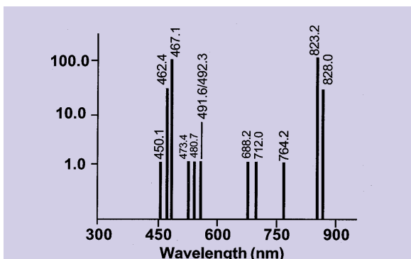
XENON SPECTRUM
