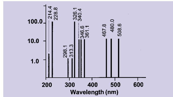
CADMIUM SPECTRUM
