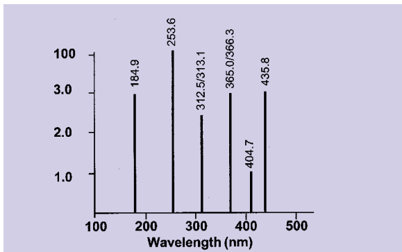
MERCURY SPECTRUM
