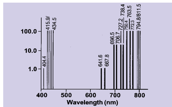
ARGON SPECTRUM
