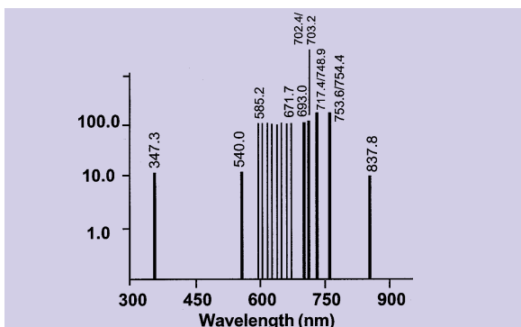
NEON SPECTRUM
