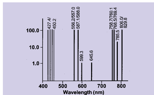
KRYPTON SPECTRUM
